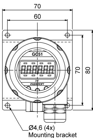
Installation drawing
